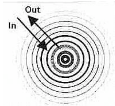
Figure 1. The spherical waves of the electron or positron.
